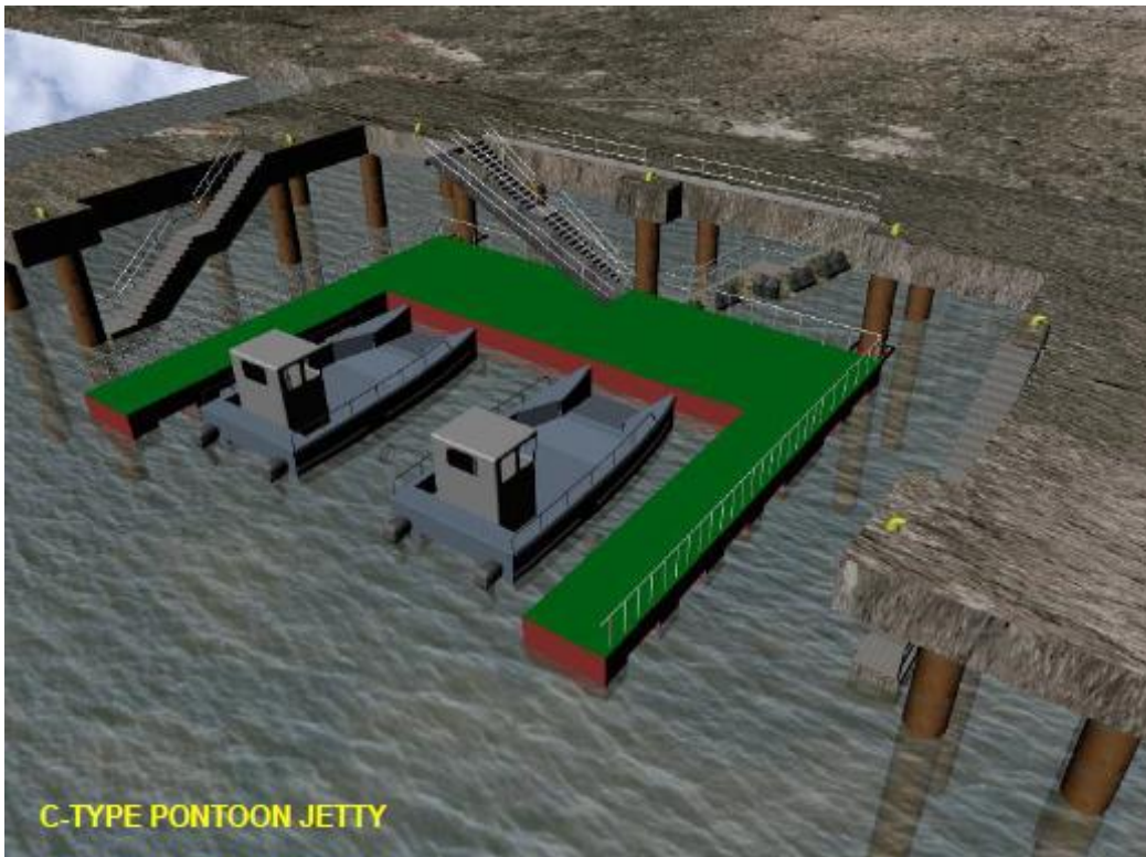
C-Type Boat Landing Jetty 3-D Concept At NSICT (Ongoing Project)
